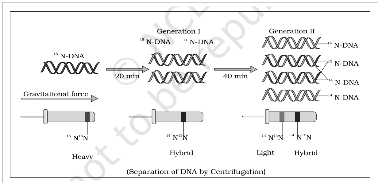
Figure 5.7 Meselson and Stahl's Experiment. Starting from ^{15}\text{N} -DNA, 20 min in ^{14}\text{N} medium gives Generation I (one ^{15}\text{N} -DNA strand with one ^{14}\text{N} -DNA strand) and 40 min gives Generation II . Under Gravitational force the tubes below show the bands -- ^{15}\text{N}^{15}\text{N} Heavy , ^{14}\text{N}^{15}\text{N} Hybrid and ^{14}\text{N}^{14}\text{N} Light -- the caption noting the Separation of DNA by Centrifugation .
