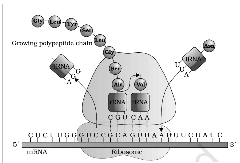
Figure 5.13 Translation. The Ribosome moves along the mRNA from 5' to 3' while each tRNA delivers its amino acid to the Growing polypeptide chain -- here the residues Gly, Leu, Tyr, Ser, Ala, Val and Asn .
